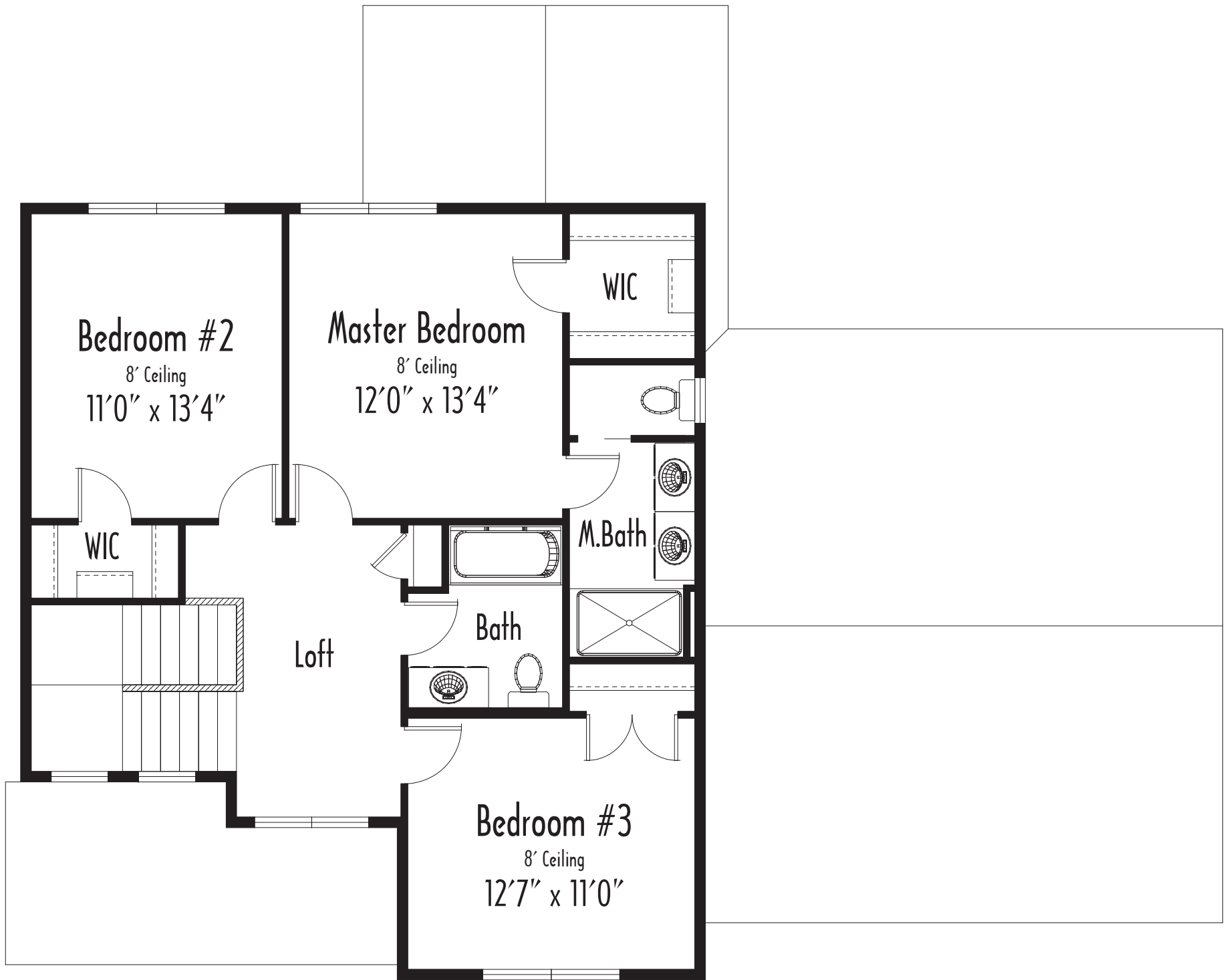
SECOND FLOOR 819 SQ.FT.
