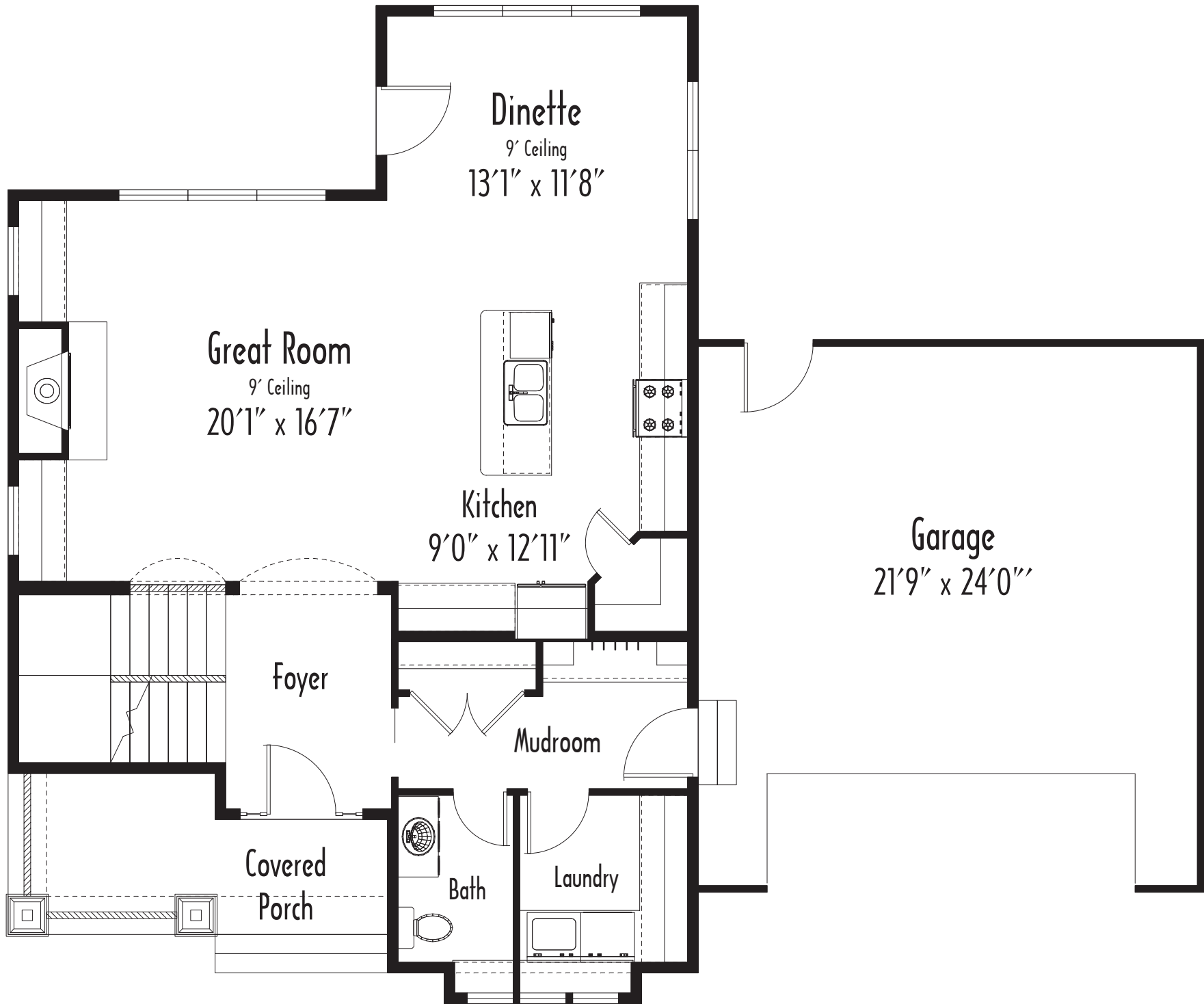
FIRST FLOOR 1,015 SQ.FT.
